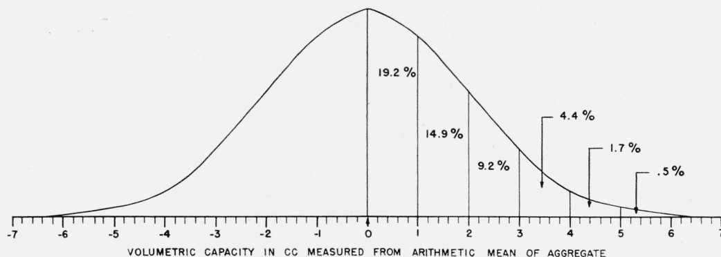
FIGURE 1. Theoretical frequency distribution of volumetric capacities of cylinders to be used for insecticide dispensers.
